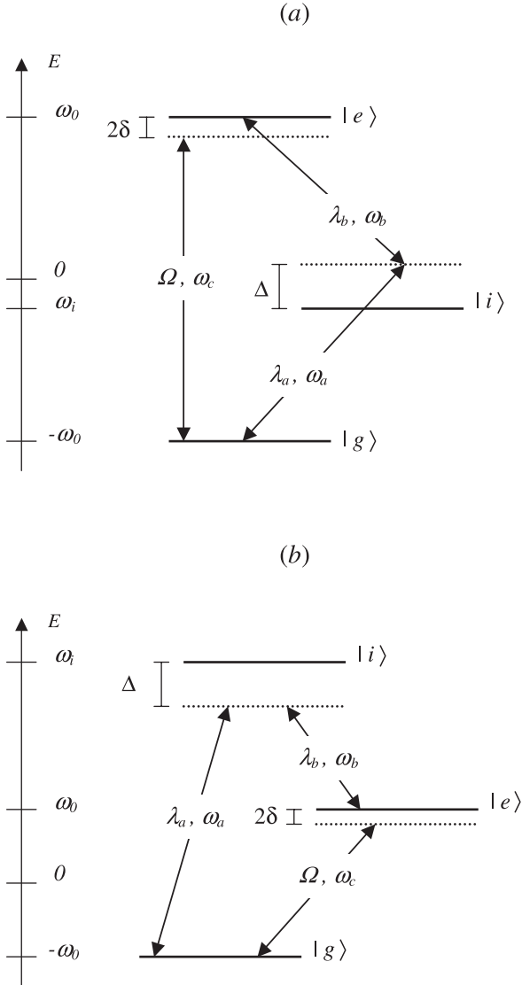
Fig. 1. Energy diagram of a three-level atomic system in the (a) ladder and (b) lambda configurations.
